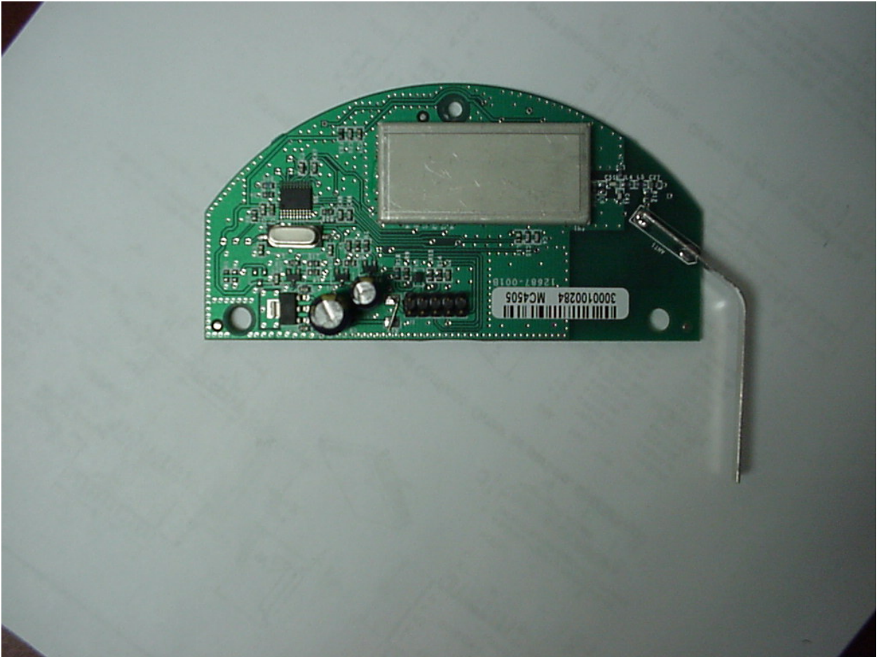
Figure 2: Internal – PCB Front View
