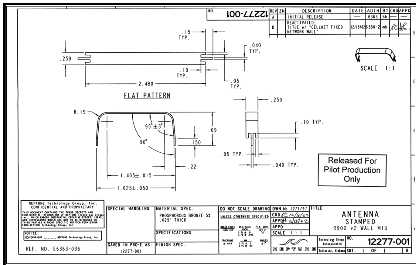
Figure E2: Drawing of New Antenna
