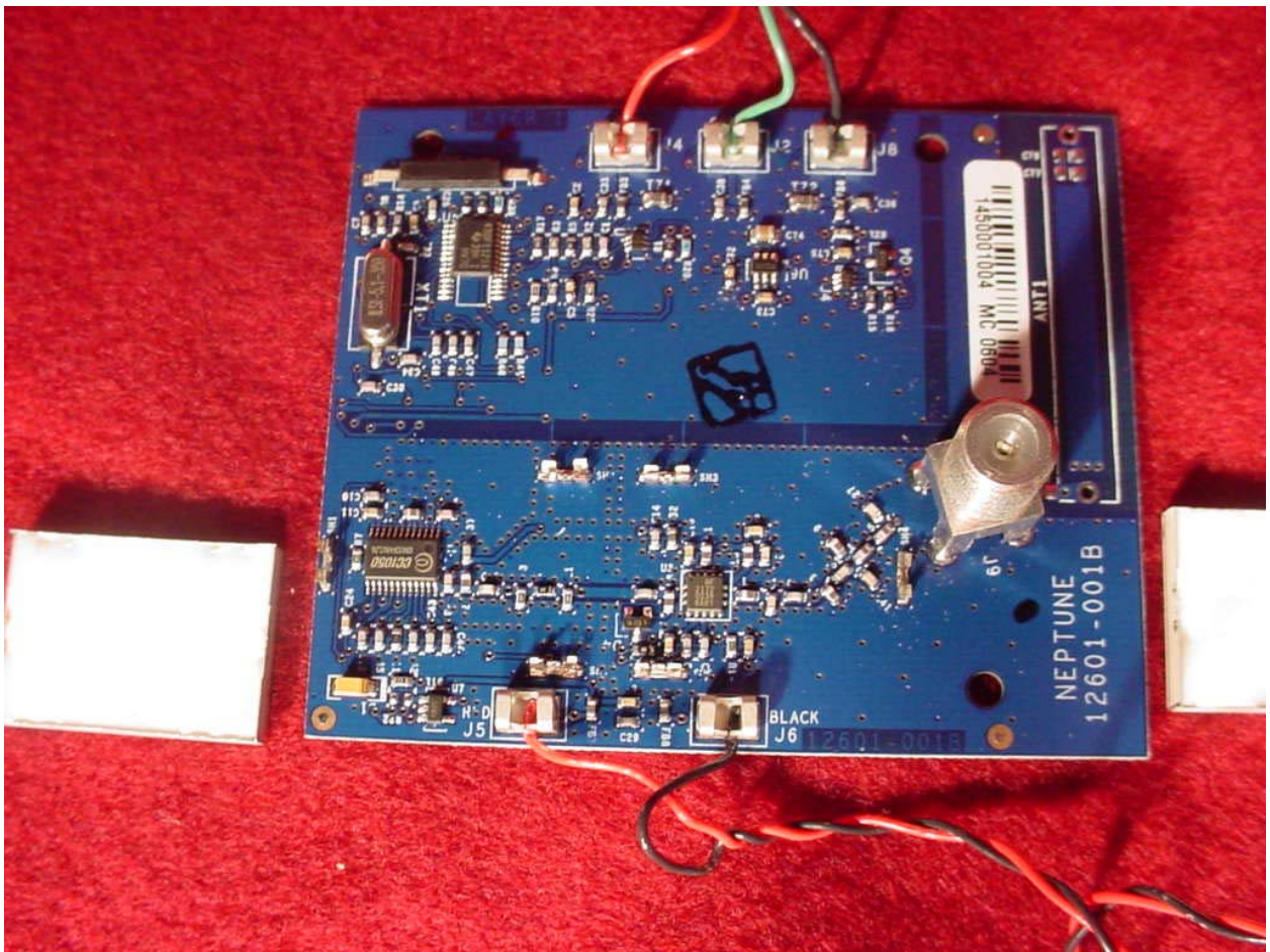
Figure 8: Shields Removed – Both Variants
