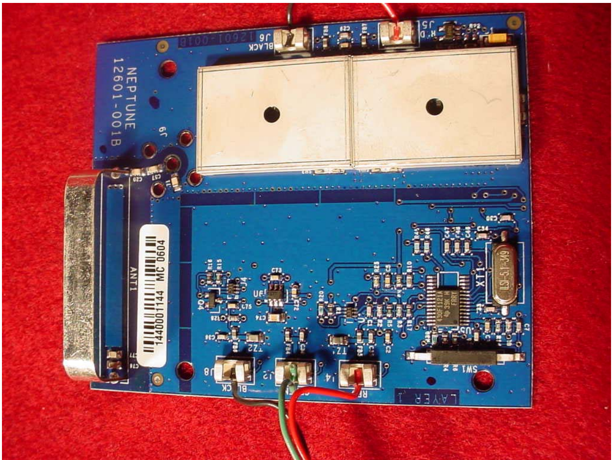
Figure 3: Wall Unit – Top of PCB
