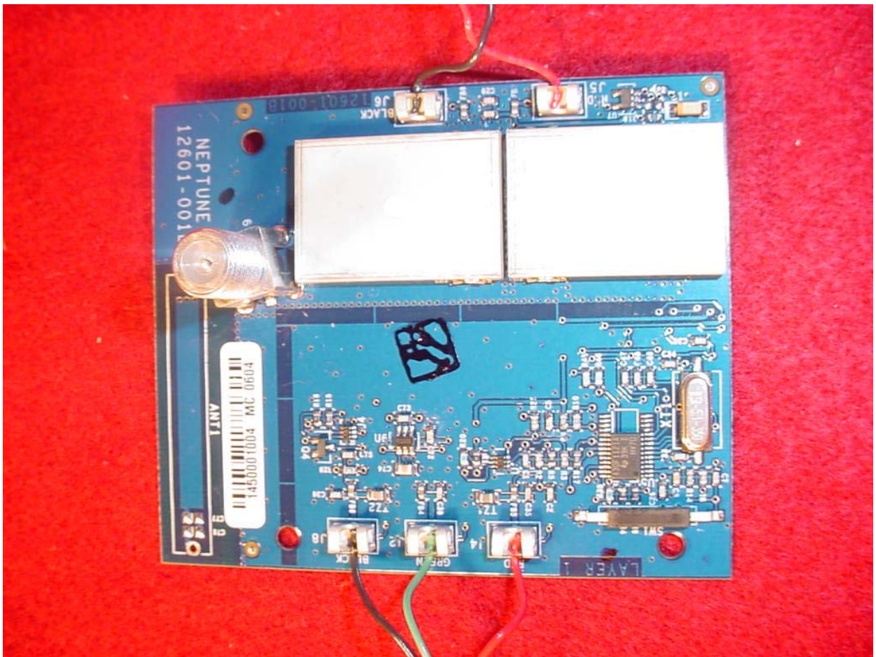
Figure 7: Pit Unit – PCB Top View
