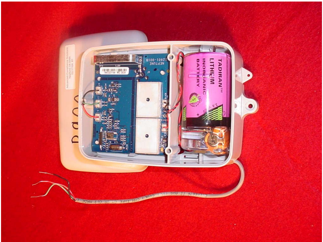
Figure 2: Wall Unit – Cover Removed
