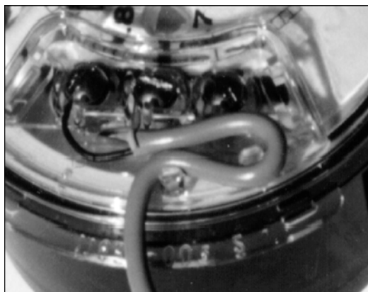
Figure 6 Cable Threaded Around Strain Relief Posts
