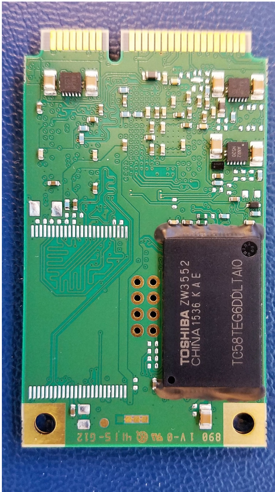
mSATA DRIVE – BOTTOM VIEW
