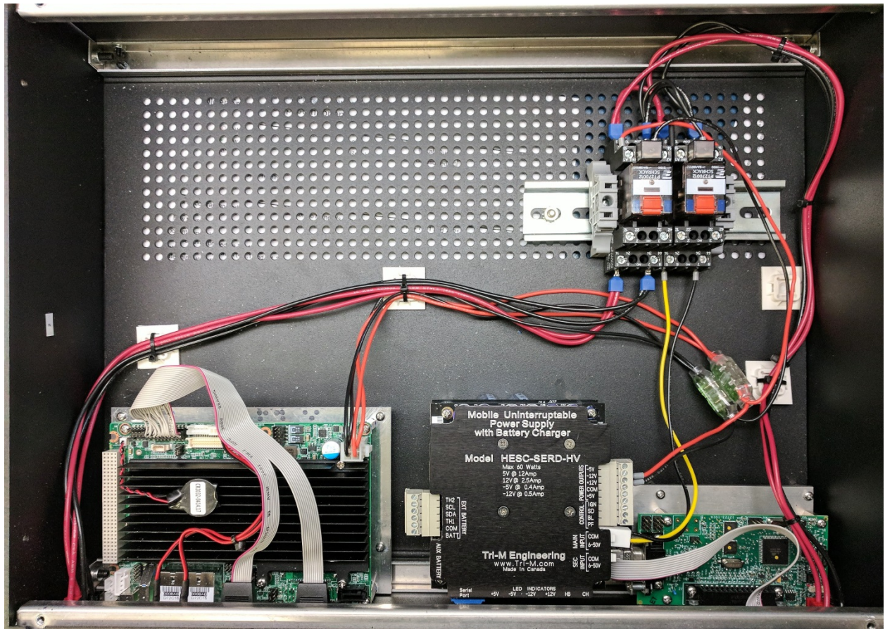
RACK MOUNT ENCLOSURE ASSEMBLY
