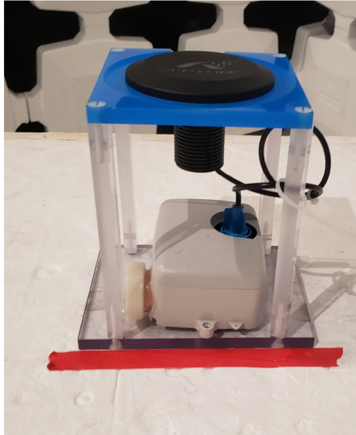
Figure 1. Pit Antenna in test jig
