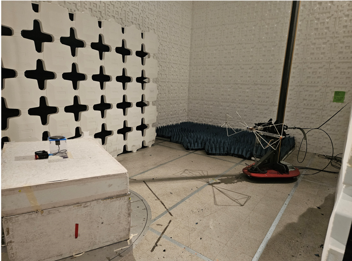
Figure 2. Radiated Emissions 30-200 MHz
