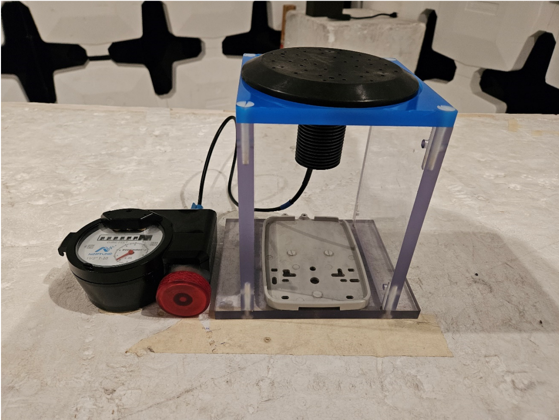
Figure 1. Pit Antenna in Test Jig
