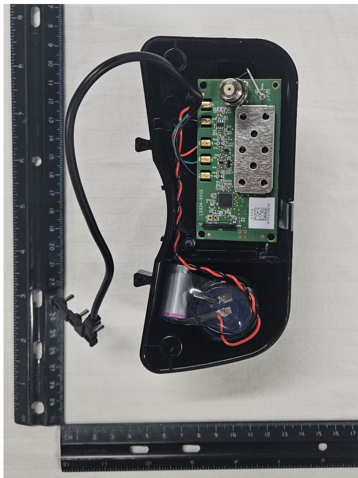
Figure 1. Host device with Cover Removed
