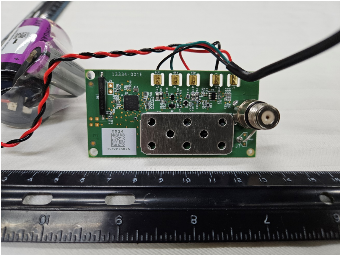
Figure 2. R900M module top side
