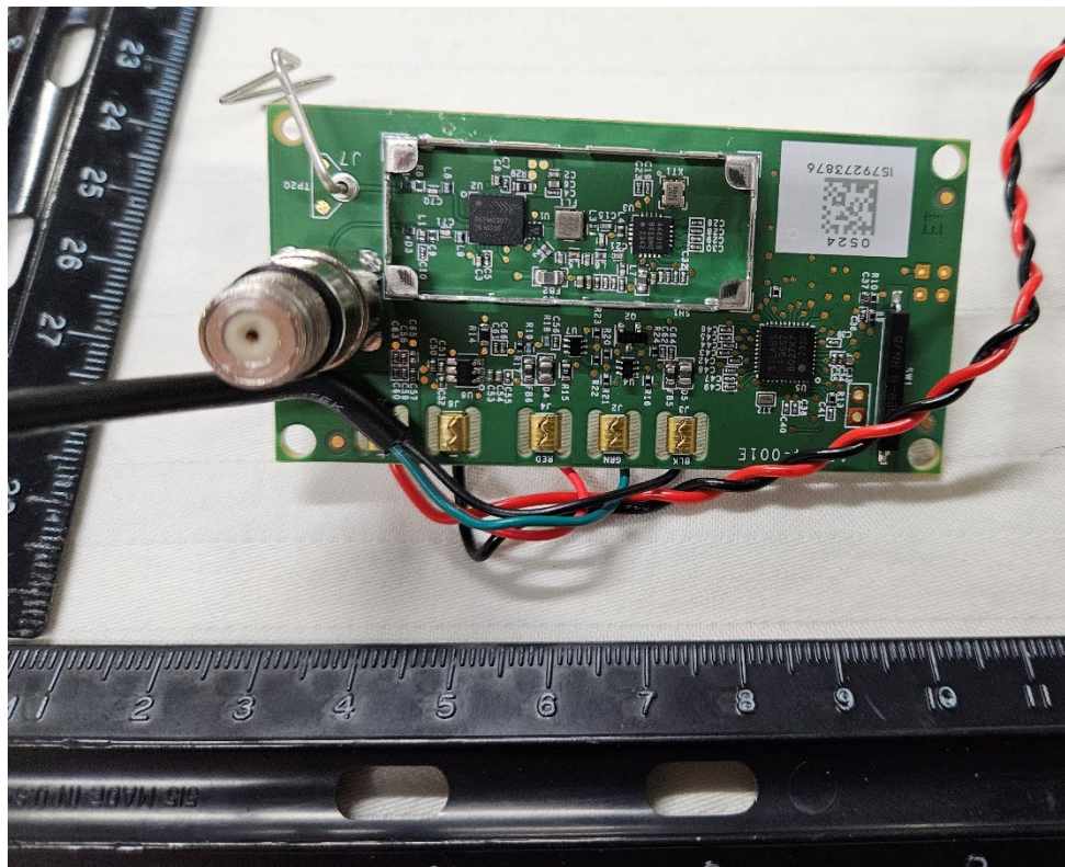
Figure 3 R900M module, Shielding Removed
