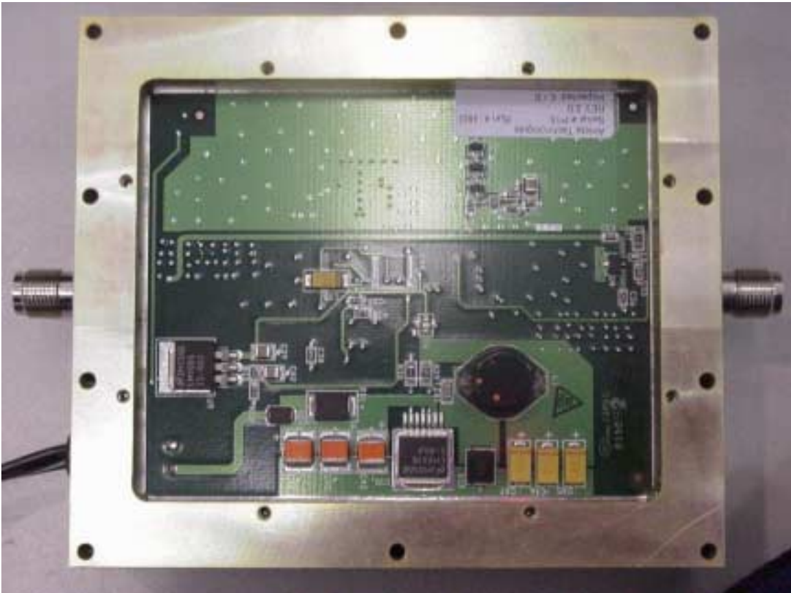
Figure 2. PCB Bottom View
