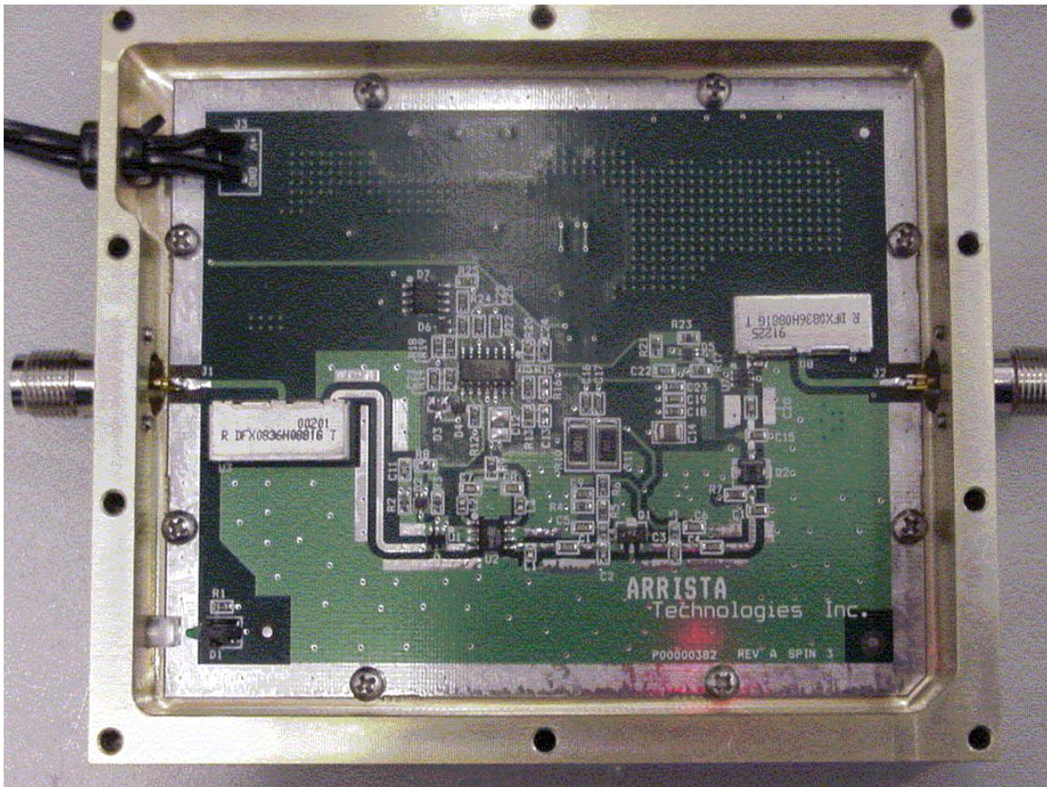
Figure 3. PCB Top View
