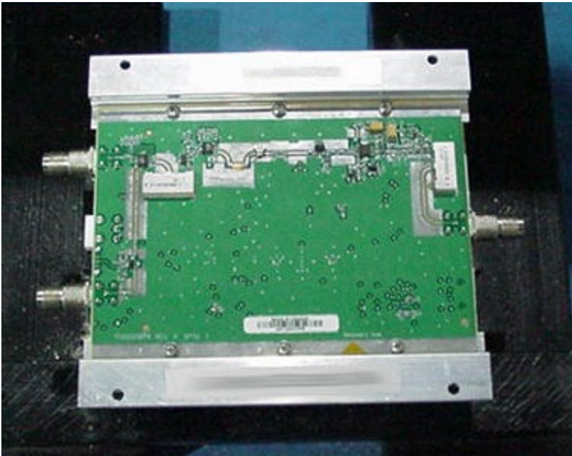
Article 02- Internal Photo: Bottom View
