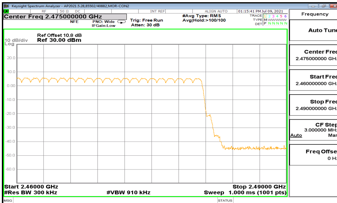
30MHz SPAN, SEGMENT 3 OF 3
