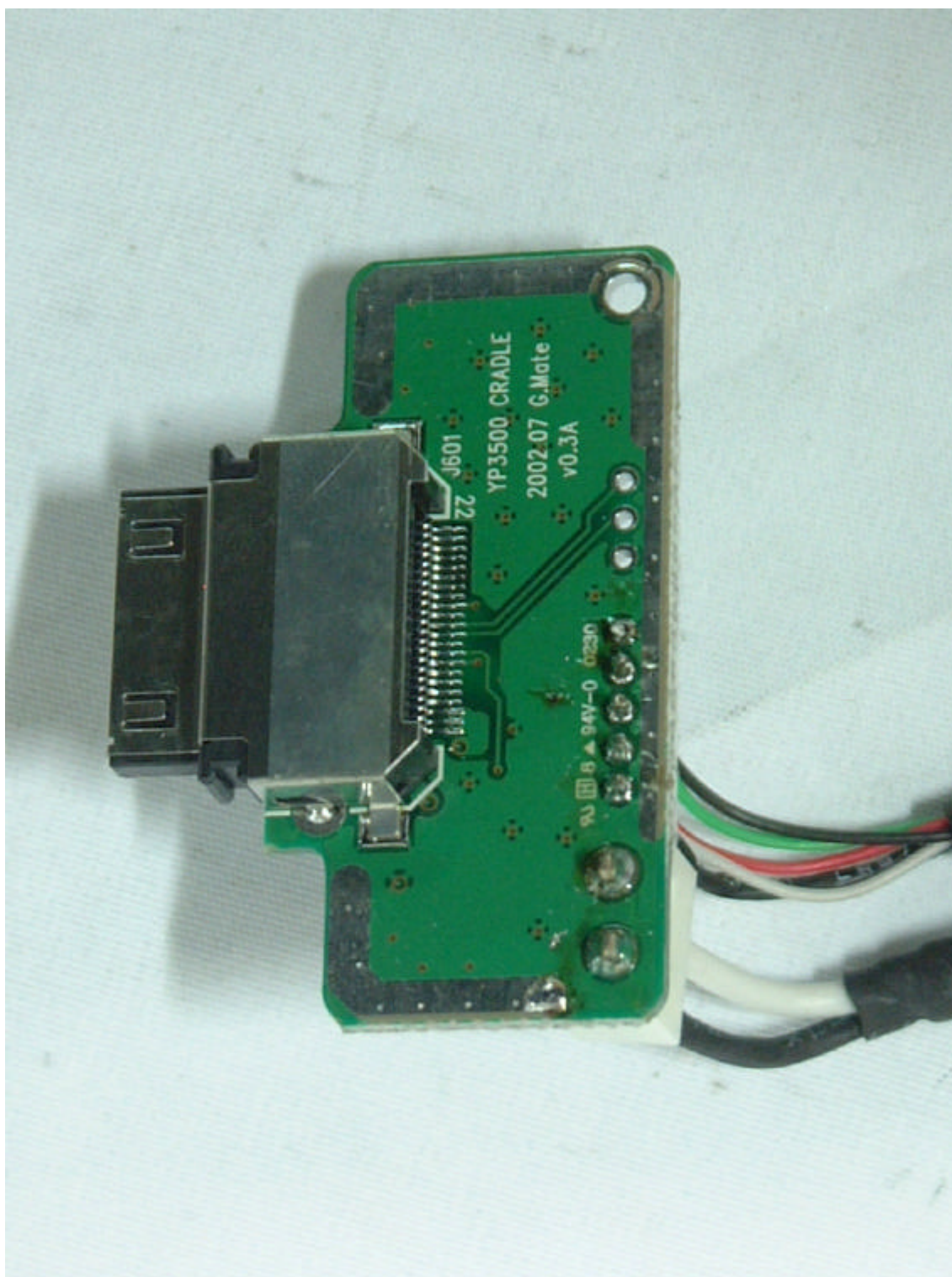
<REAR VIEW OF CRADLE BOARD>
