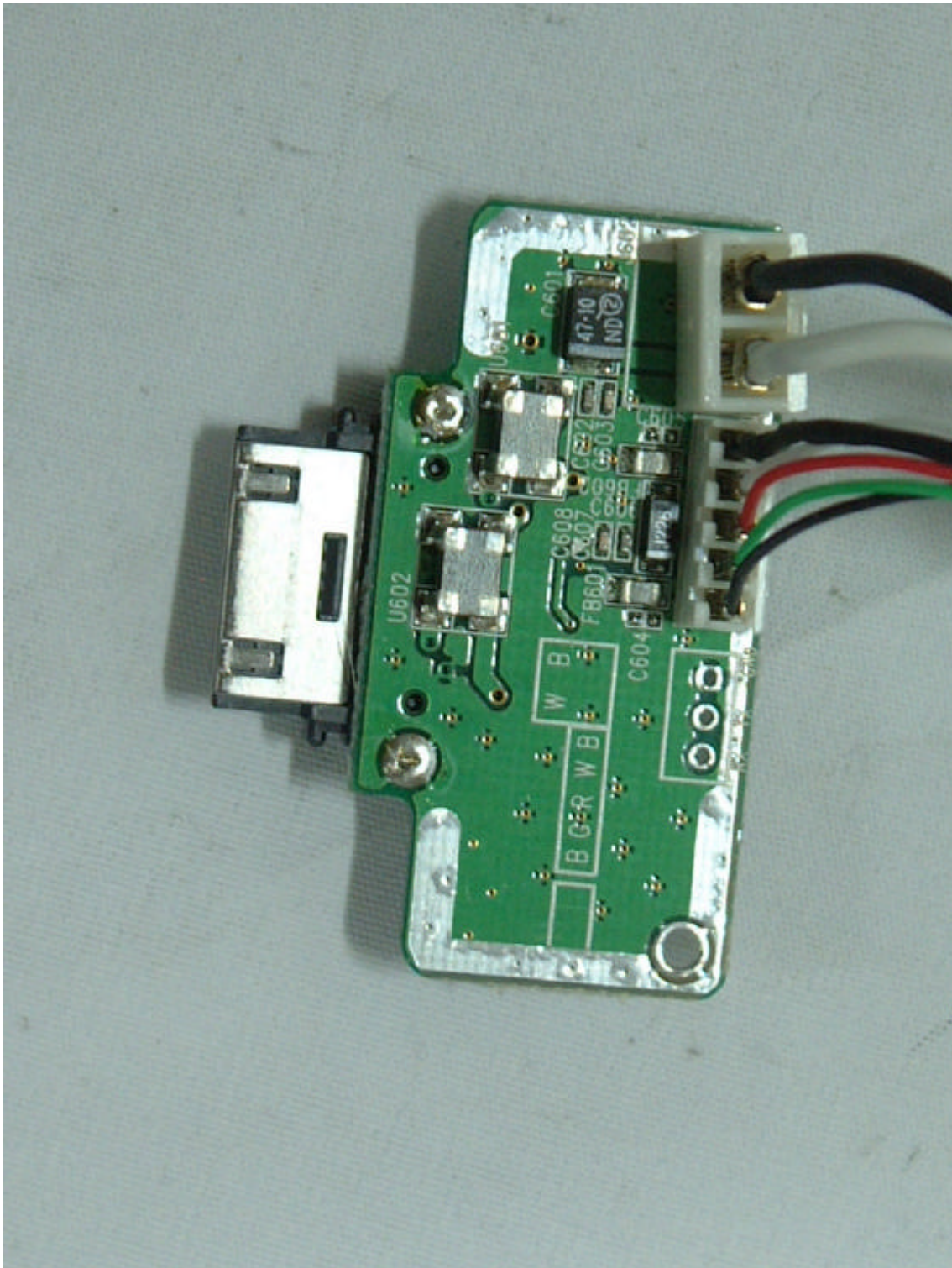
<FRONT VIEW OF CRADLE BOARD>
