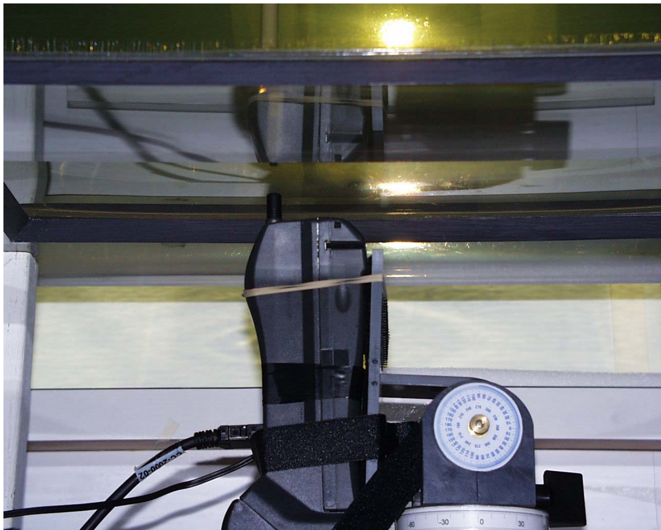
< Top face toward phantom, tip of antenna in contact and antenna fully retracted >
