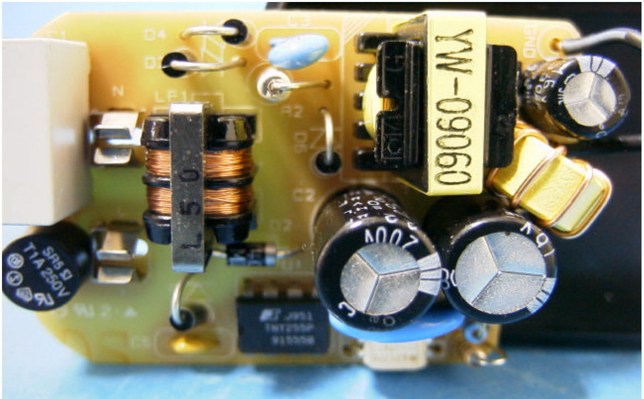
Parts Side of Powerboard
