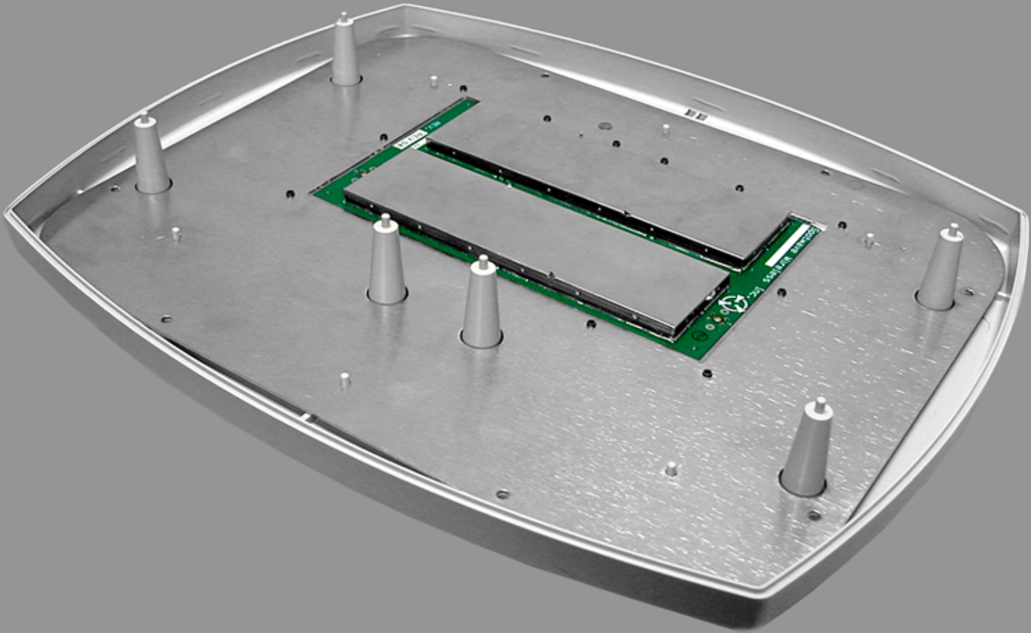
DDU - OVERALL INTERNAL VIEW
