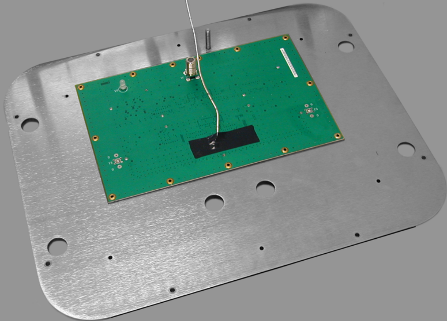
DDU - INTERNAL VIEW TRACK SIDE OF RADIO CIRCUITRY
