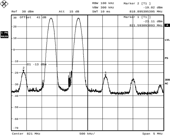
Uplink - 4FSK - 3rd Order Intermodulation Date: 9.NOV.2006 19:24:25
