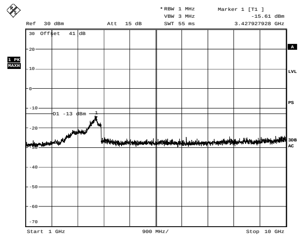
Uplink - 4FSK - High Channel - Conducted Emissions Date: 9.NOV.2006 19:26:56
