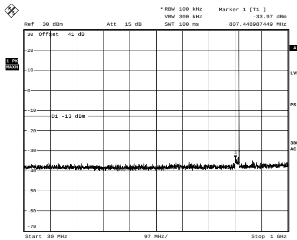
Uplink - 4FSK - High Channel - Conducted Emissions Date: 9.NOV.2006 19:26:32
