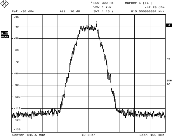
Uplink - 4FSK - Input Date: 9.NOV.2006 19:06:10
