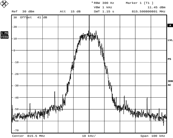
Uplink - 4FSK - Output Date: 9.NOV.2006 19:04:41
