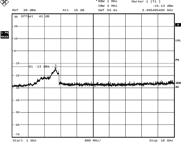
Uplink - 4FSK - Low Channel - Conducted Emissions Date: 9.NOV.2006 19:29:40
