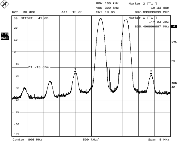
Uplink - 4FSK - 3rd Order Intermodulation Date: 9.NOV.2006 19:15:40
