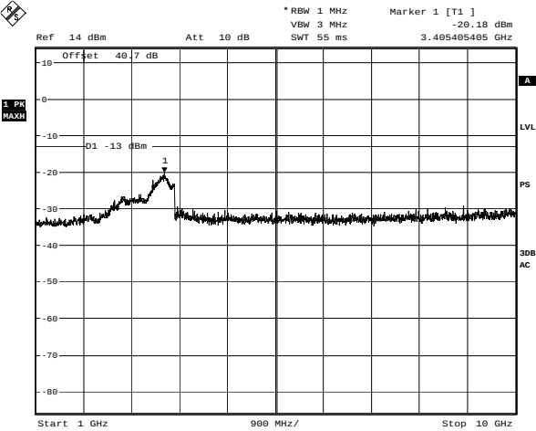
Downlink - 4FSK - Low Channel - Conducted Emissions Date: 9.NOV.2006 16:13:25
