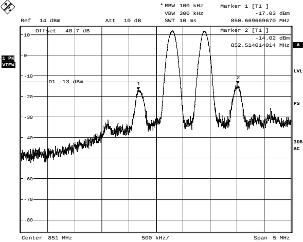
Downlink - 4FSK - 3rd order Intermodulation Date: 9.NOV.2006 16:11:09
