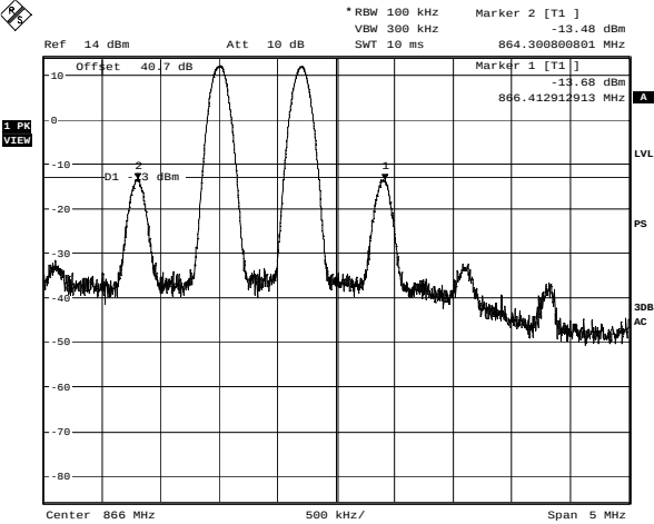
Downlink - 4FSK - 3rd order Intermodulation Date: 9.NOV.2006 16:04:07
