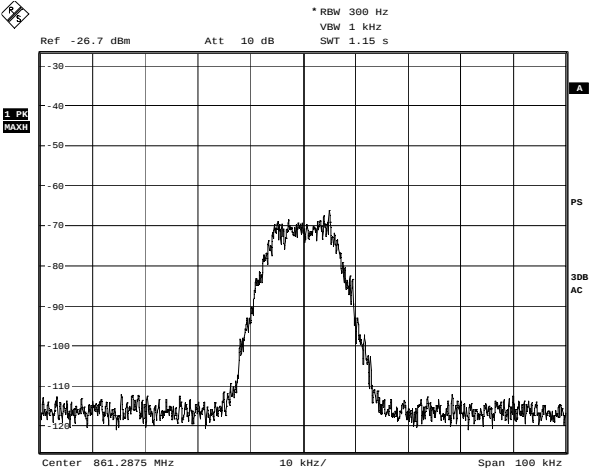
Downlink - 4FSK Input Date: 9.NOV.2006 15:15:56
