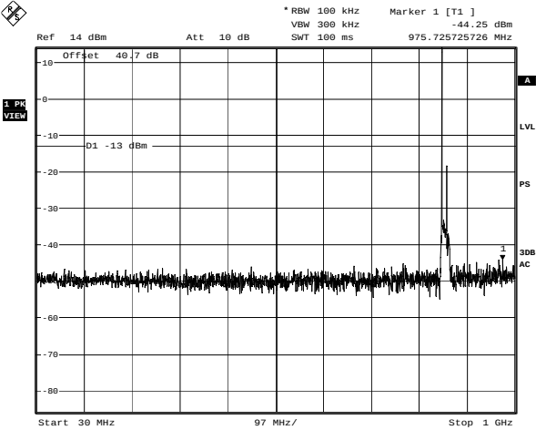
Downlink - 4FSK - Low Channel - Conducted Emissions Date: 9.NOV.2006 16:12:56
