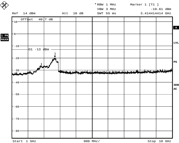
Downlink - 4FSK - Mid Channel - Conducted Emissions Date: 9.NOV.2006 16:17:35
