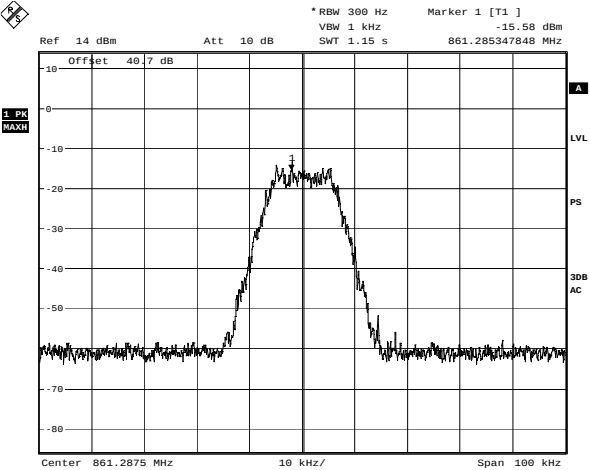
Downlink - 4FSK Output Date: 9.NOV.2006 15:14:38
