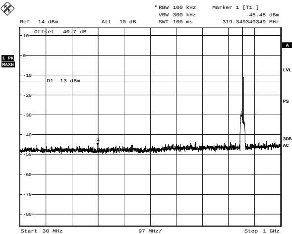
Downlink - 4FSK - Mid Channel - Conducted Emissions Date: 9.NOV.2006 16:16:14
