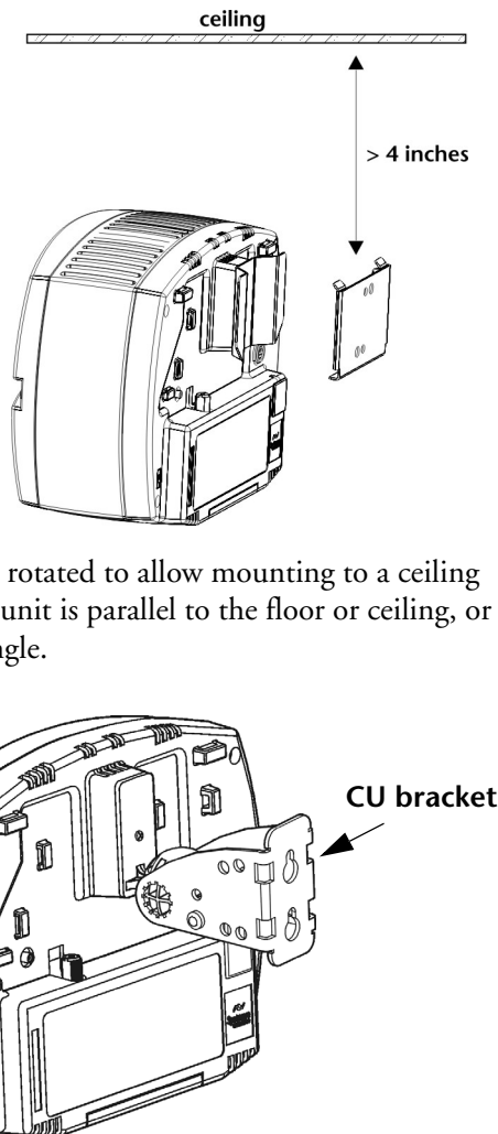
Figure 3.9: Optional CU mounting bracket.
