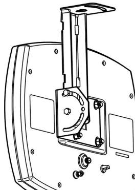
Figure 3.2: Overhead mounting arrangement
