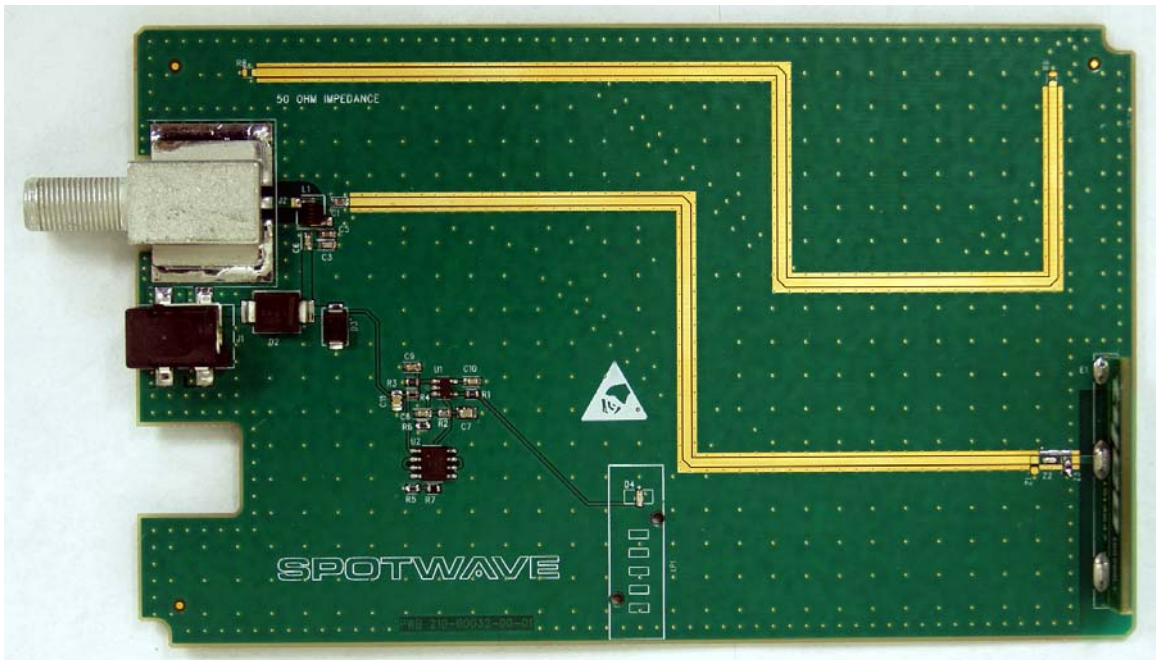
PCB – Top
