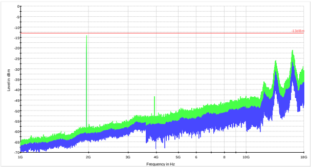
Figure 8.5-2: DL 1-18 GHz
