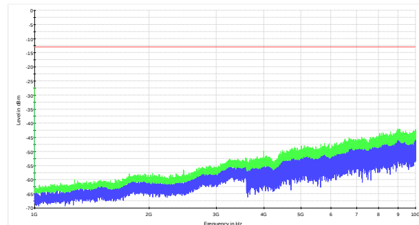
Figure 8.6-2: DL 1-10 GHz
