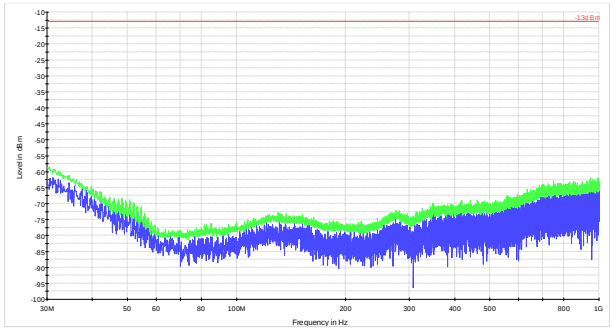
Figure 8.5-1: DL 30-1000 MHz
