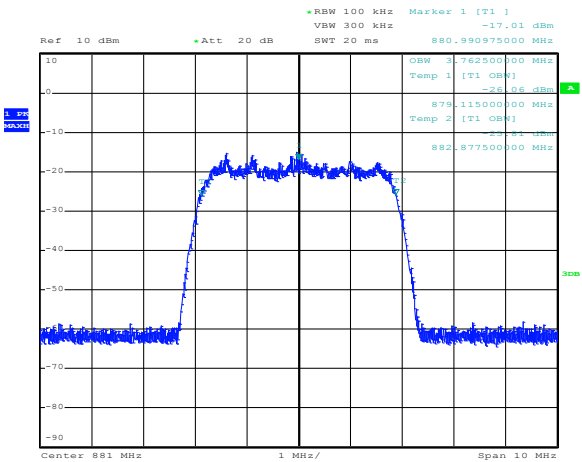
Figure 8.7-14: Cell CDMA 3xRTT DL output
