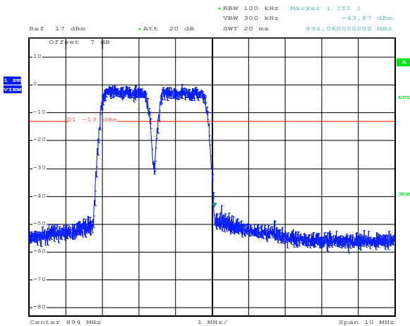
Figure 8.4-9: GSM DL Upper Band edge
