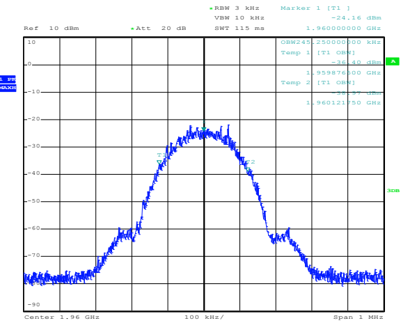
Figure 8.7-8: PCS GSM DL output
