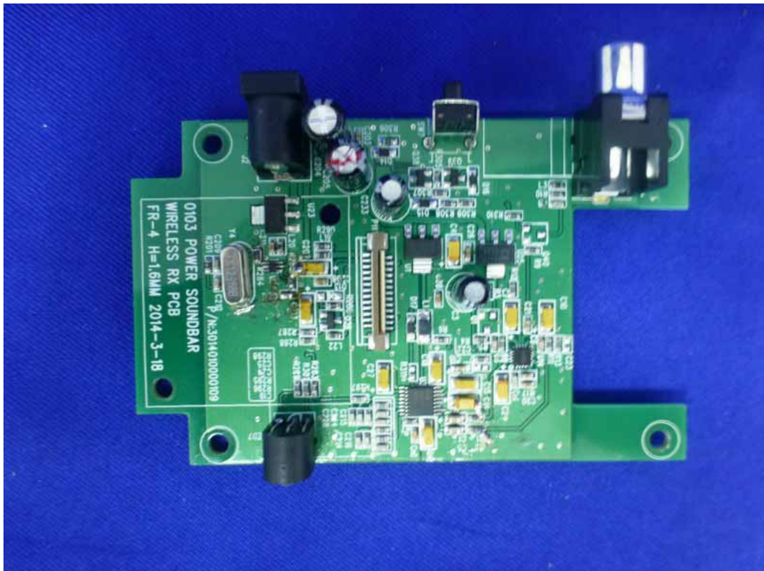
Figure 14 Inside of the PCB
