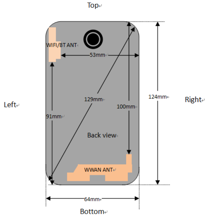
Fig.14.1 EUT Antenna Locations
