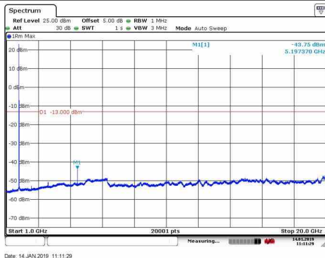
Band4_20MHz_16QAM_20300_1RB#0
