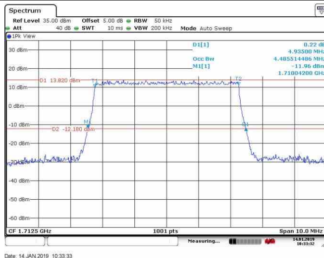
Band4_5MHz_16QAM_20175_25RB#0
