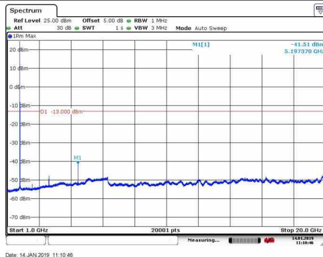
Band4_20MHz_QPSK_20300_1RB#0
