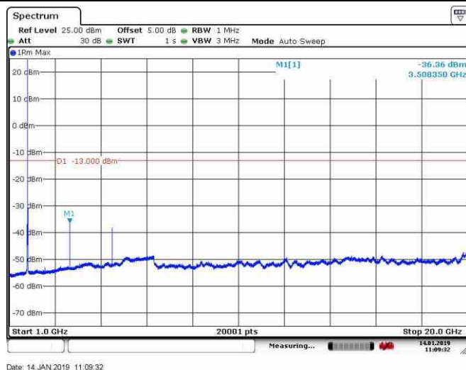
Band4_20MHz_16QAM_20050_1RB#0
