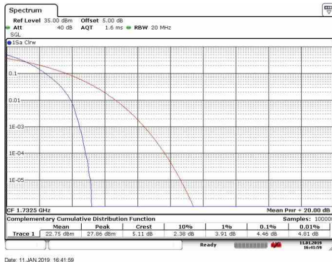
Band4_20MHz_QPSK_20300_100RB#0
