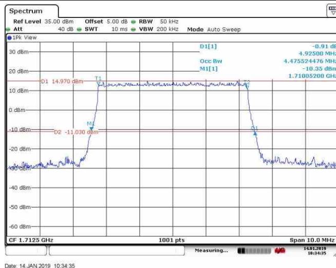
Band4_5MHz_QPSK_20175_25RB#0
