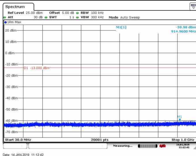
Band4_20MHz_16QAM_20175_1RB#0
