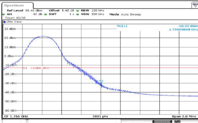
Band4-10MHz-QPSK-20350-50RB#0
