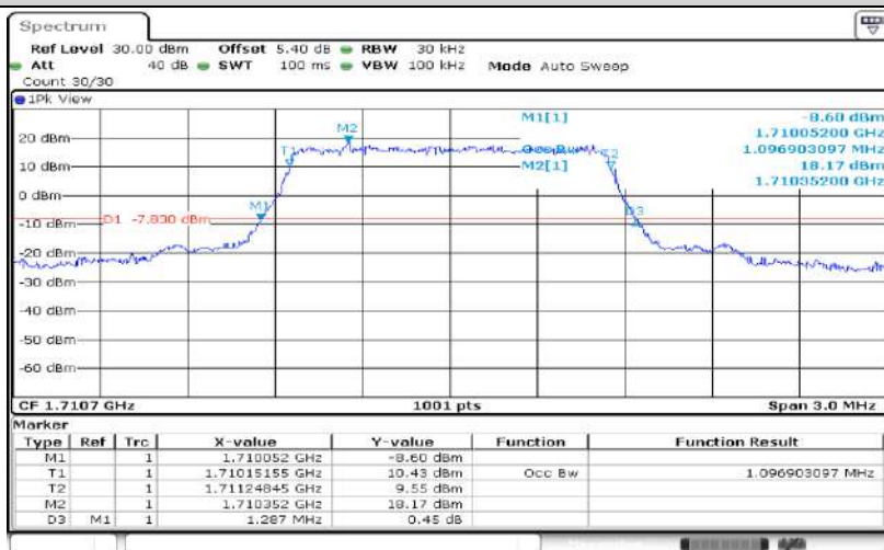
Band4-1.4MHz-QPSK-19957-6RB#0-1.097
