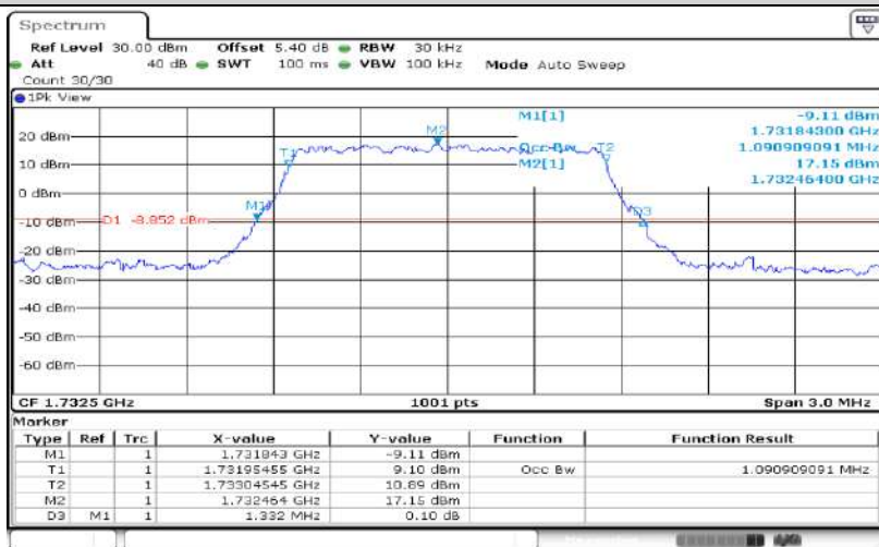
Band4-1.4MHz-QPSK-20175-6RB#0-1.091
