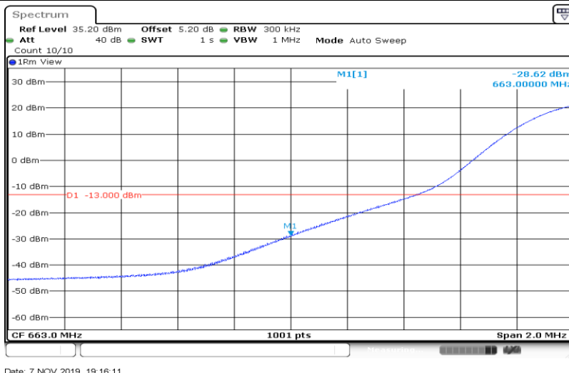
Band71-20MHz-16QAM-133222-100RB#0
