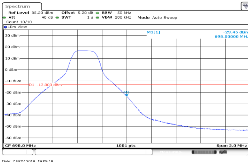
Band71-5MHz-16QAM-133447-25RB#0
