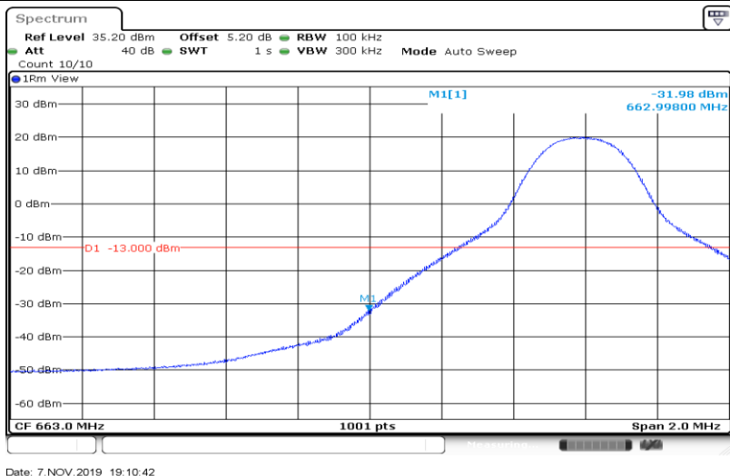
Band71-10MHz-16QAM-133172-50RB#0
