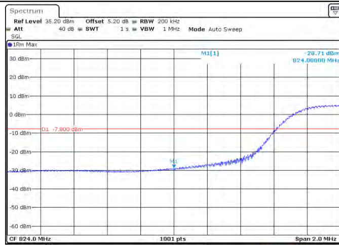
Band 26_15MHz_16QAM_26865_75RB#0
