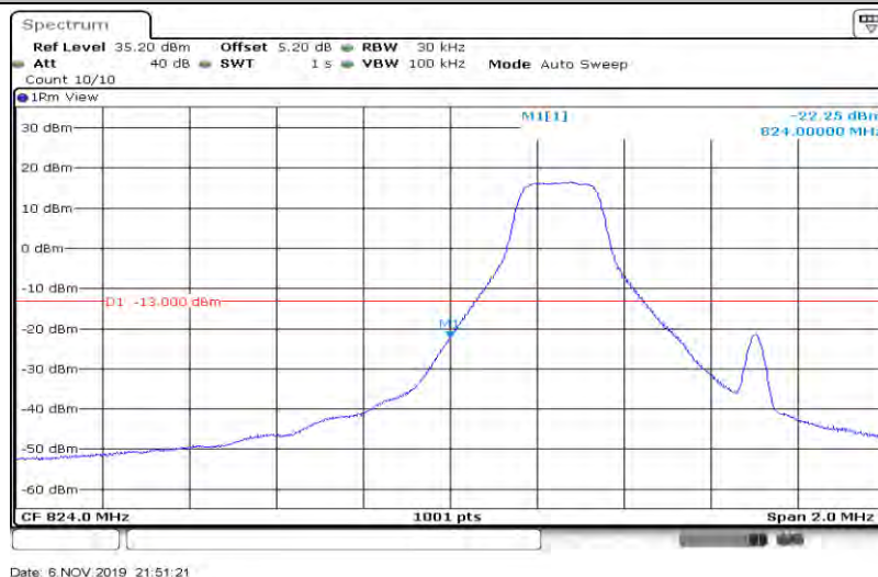
Band 26_1.4MHz_QPSK_26797_6RB#0
