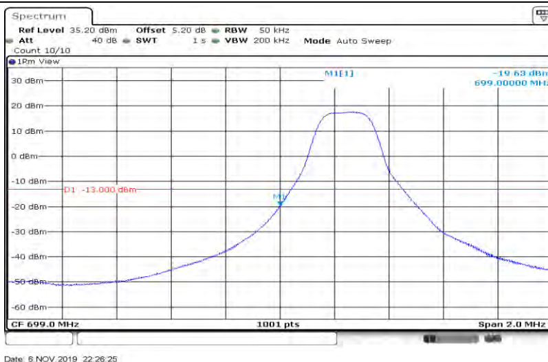
Band12-3MHz-16QAM-23025-15RB#0
