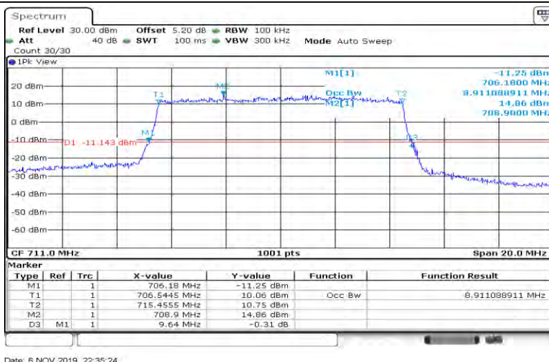
Band12-10MHz-16QAM-23060-50RB#0-8.911
