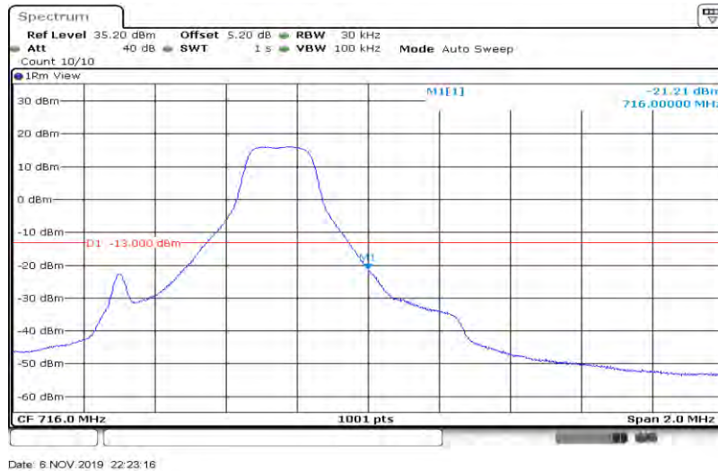
Band12-1.4MHz-16QAM-23173-6RB#0
