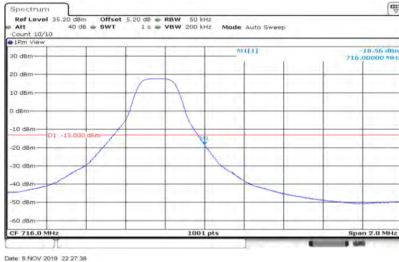
Band12-3MHz-16QAM-23165-15RB#0
