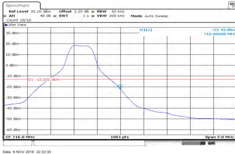
Band12-5MHz-QPSK-23155-25RB#0
