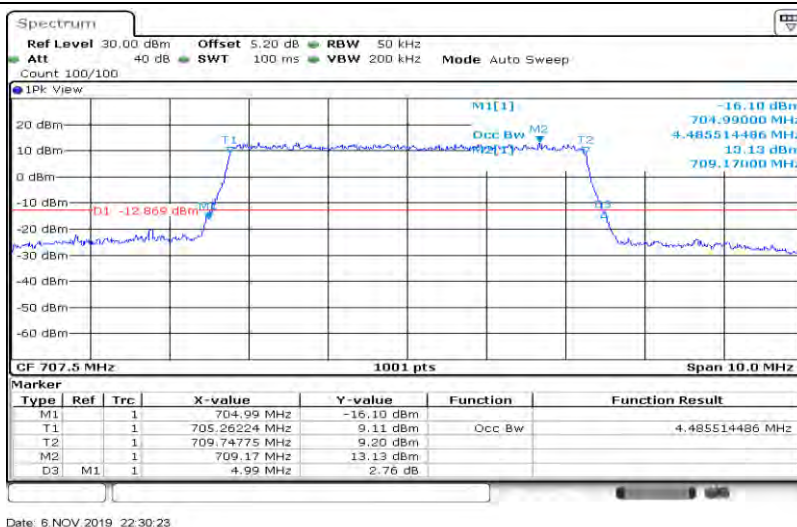
Band12-5MHz-16QAM-23155-25RB#0-4.476
