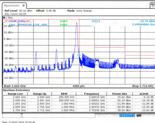
Band41_15MHz_16QAM_41515_75RB#0
