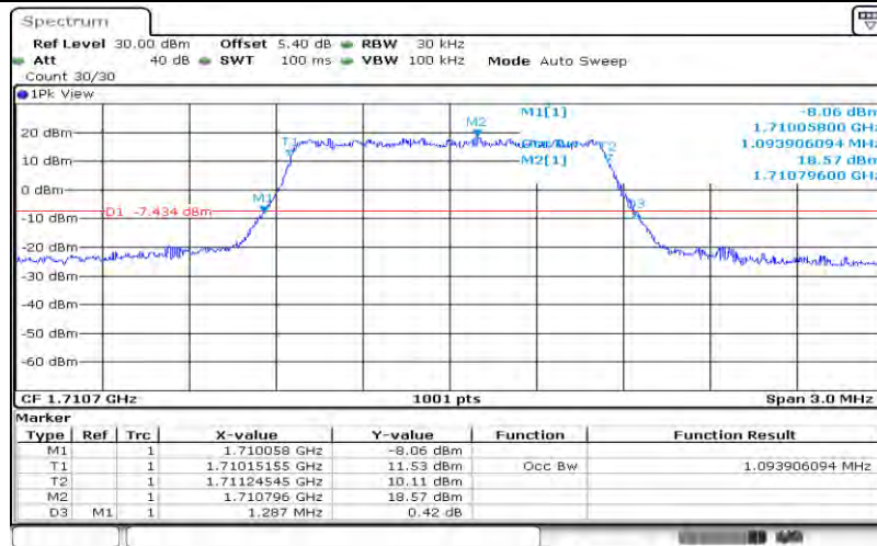
Band66-1.4MHz-QPSK-131979-6RB#0-1.094
