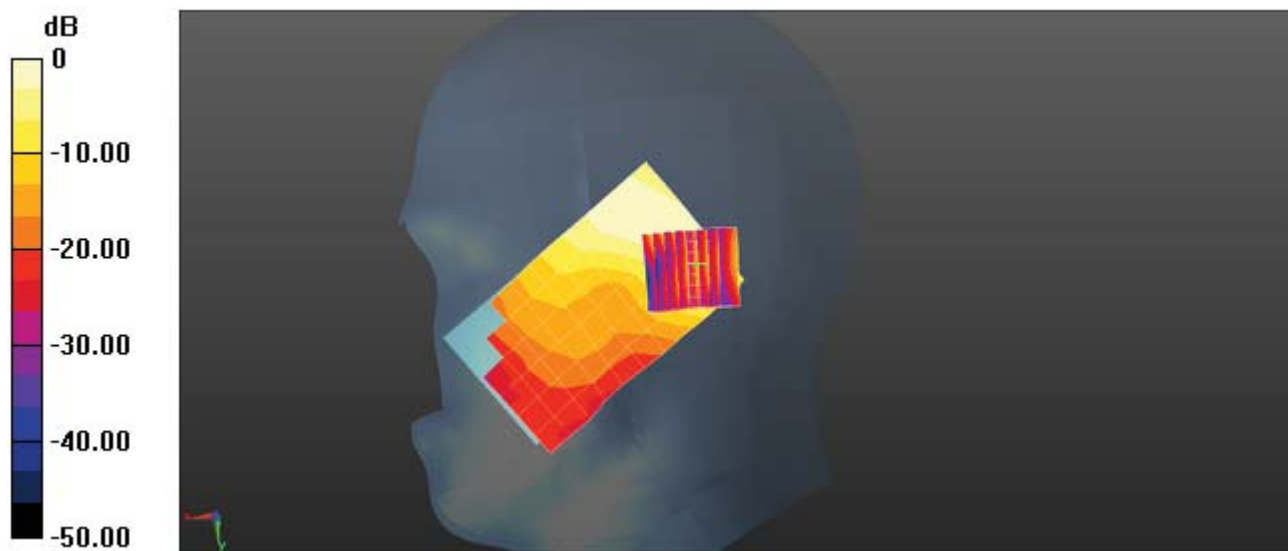
Figure 9: Right Head Cheek 802.11b Channel 6
