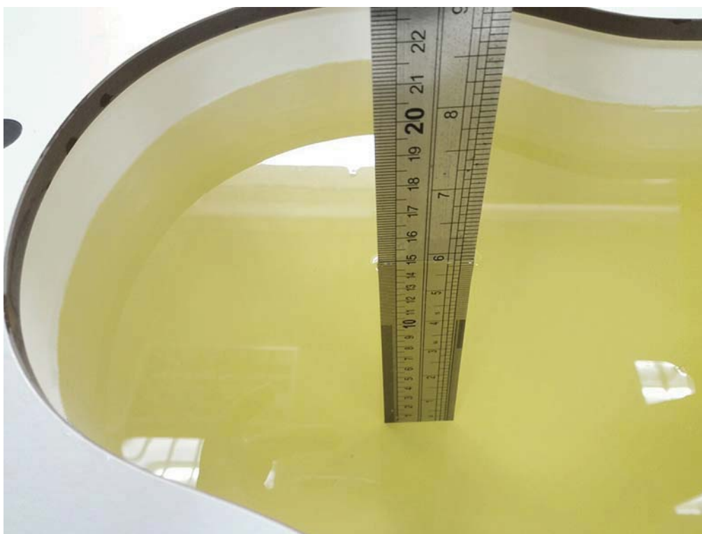
Liquid depth in the head Phantom (835 MHz, 15.0cm depth)
