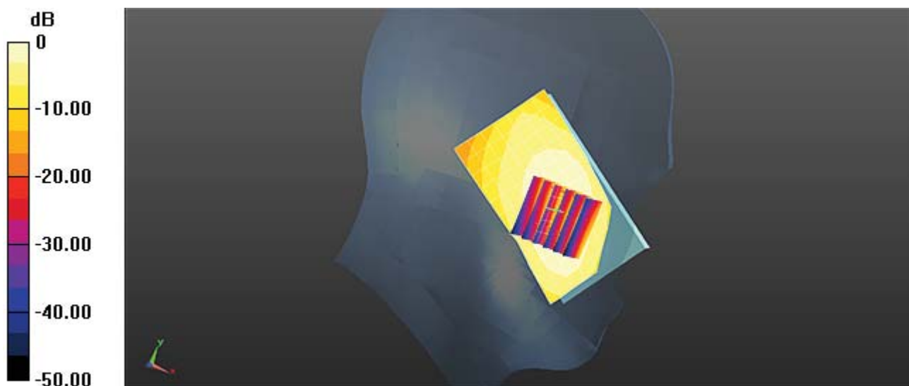
Figure 1 Left Cheek GSM 850 GPRS (2Txslots) Channel 190
