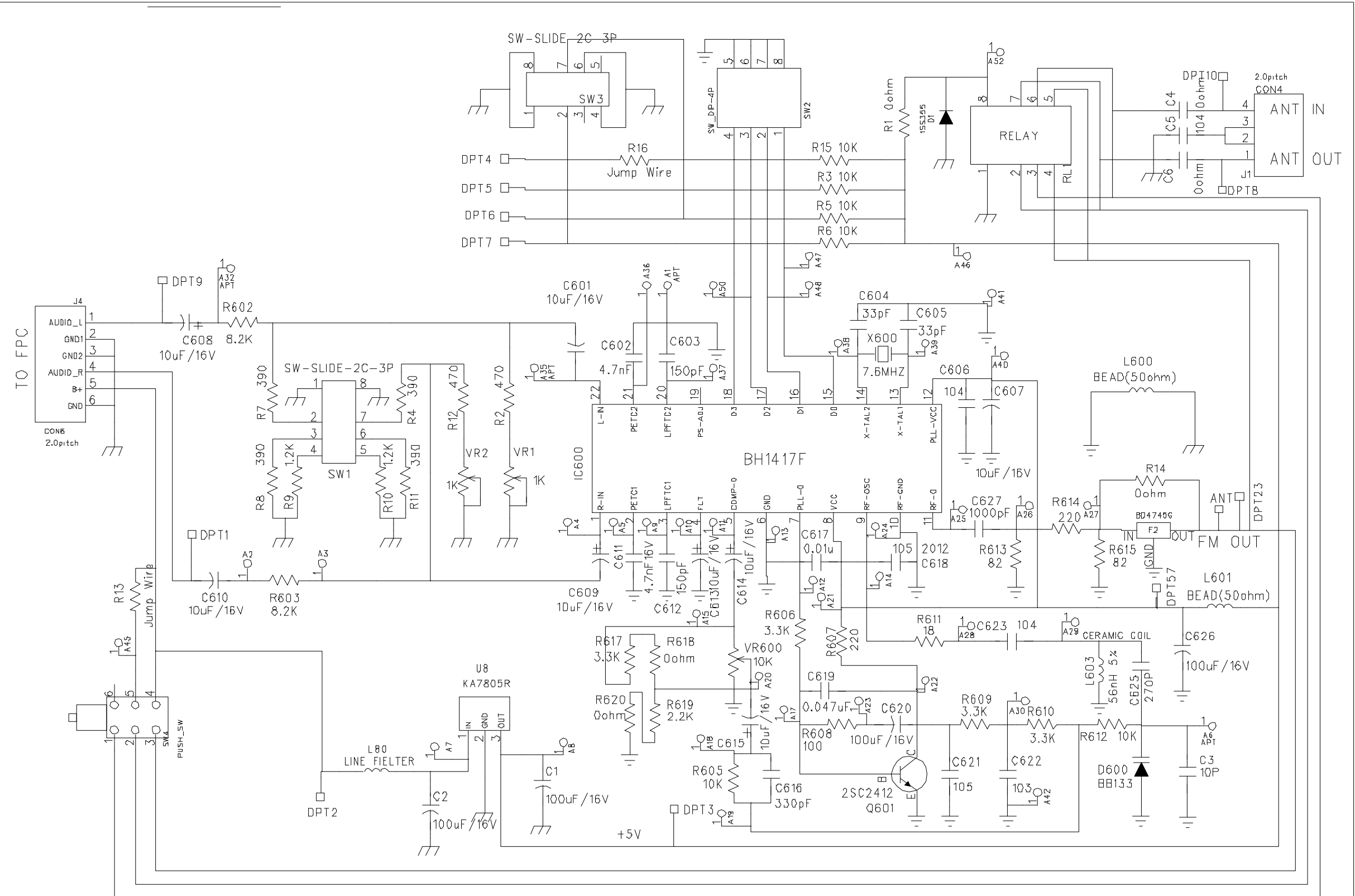
FM MODULATOR DESIGN BY B G HONG 2001.07.27
