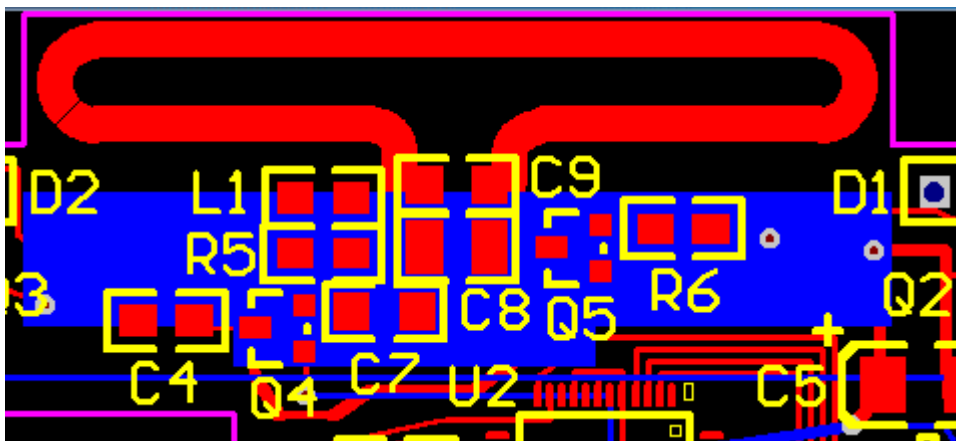
Board layout of RF transmitter portion of design
