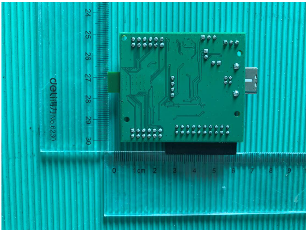
Rearview of the EUT (FLC-BTM020IQ2D) & Test Fixture
