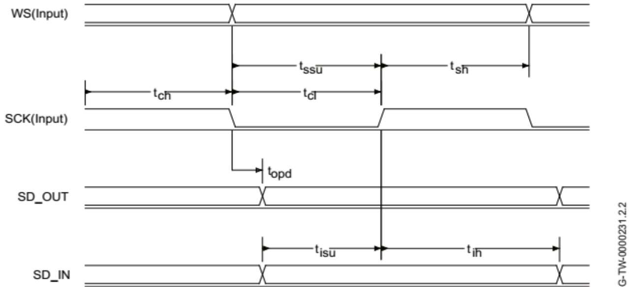
Figure 9: Digital Audio Interface Slave Timing
