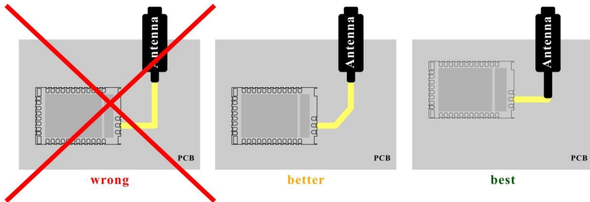
Figure 14: Recommended Trace Connects Antenna and the Module
