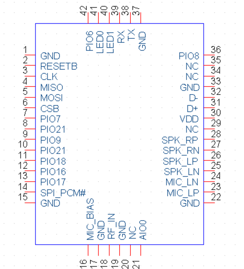
Figure 2: Pin Configuration
