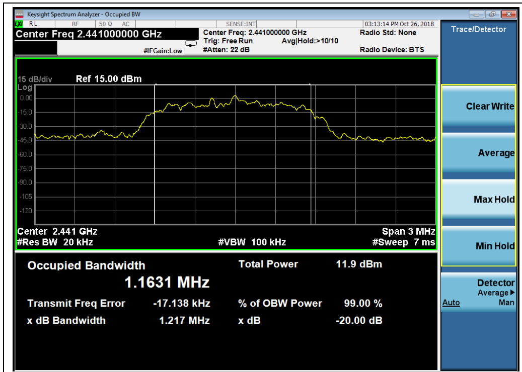
( \pi/4 -DQPSK, Channel 39, 2441MHz)
