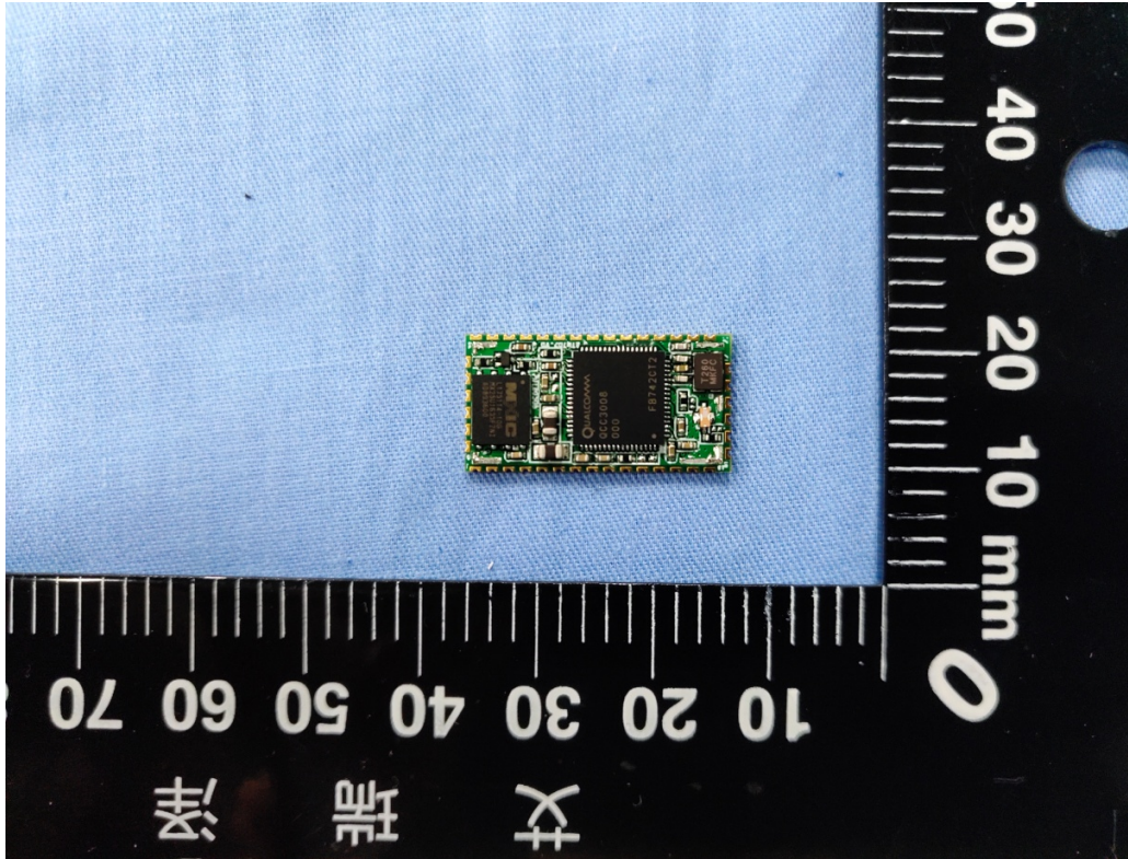
2. RF chip view
