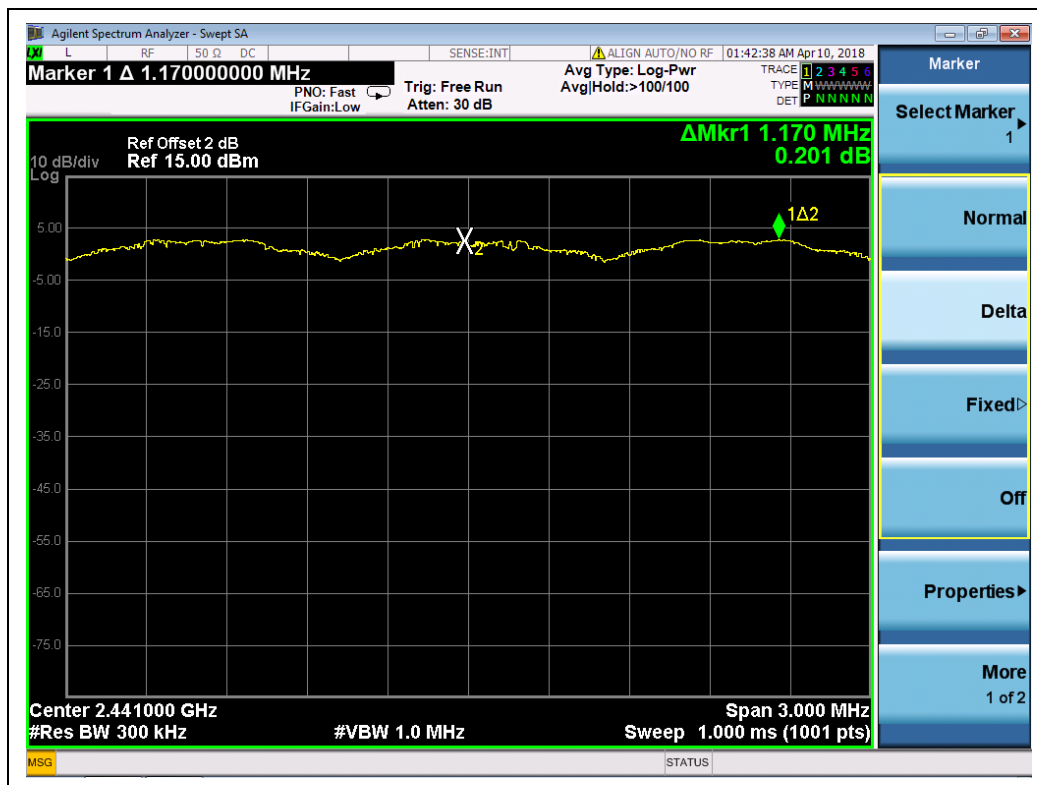
(8\text{-DPSK})
