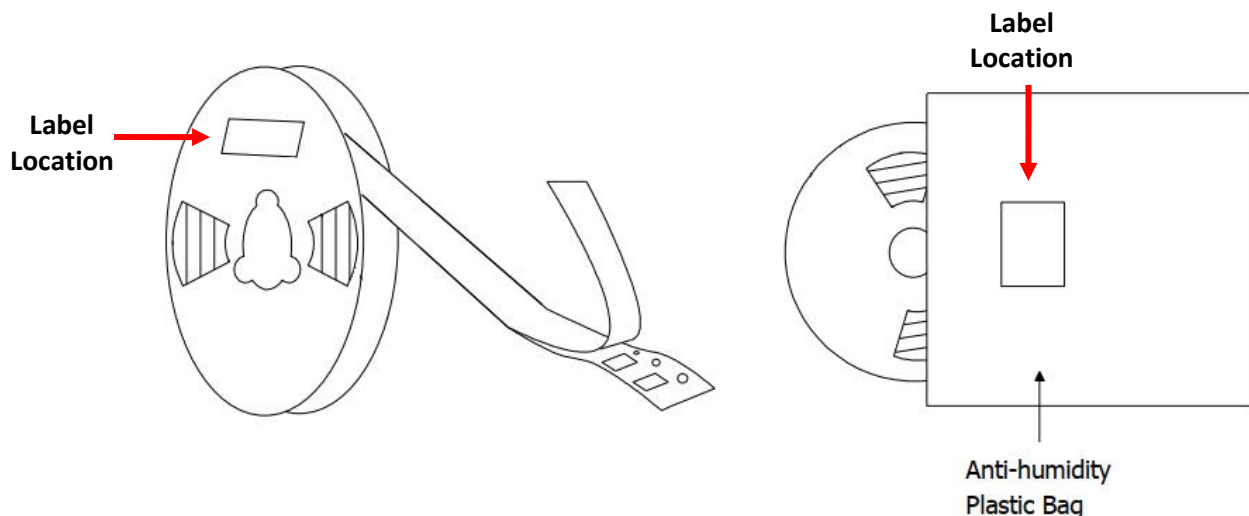
FLC-BTM901 Series Label Location
