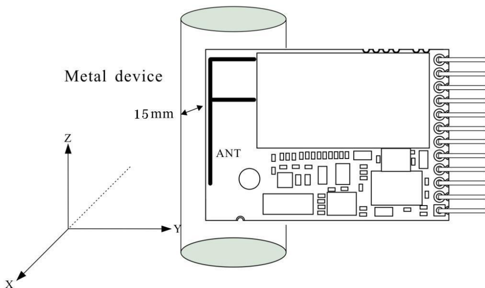
Figure 7: Leave 15mm Clearance Space from the Module Built-in Antenna
