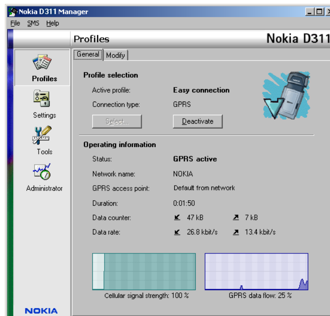
Figure 5 – Manager window
