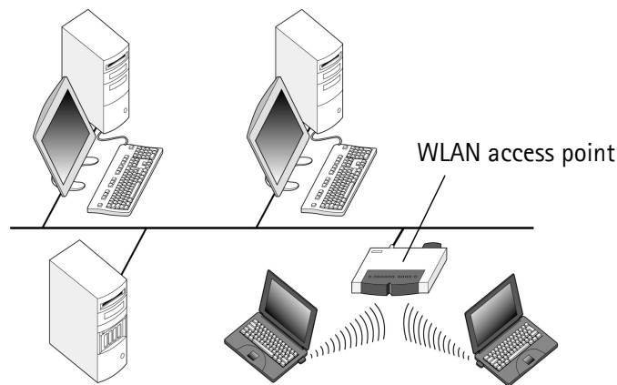
Figure 1 – Infrastructure network
