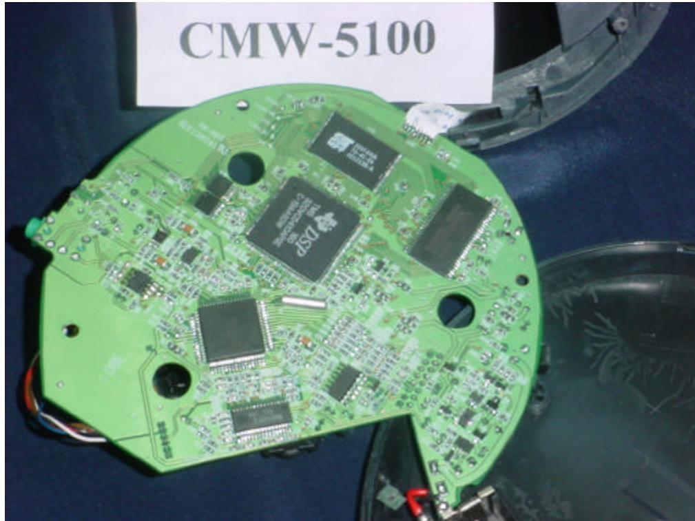
Figure 4 Inside of the EUT
