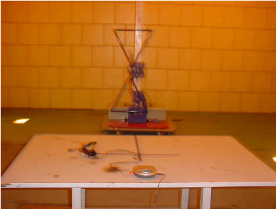
Photo of Radiated Emission Test(In Anechoic Chamber)
