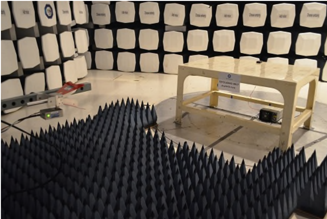
Radiated Emissions Above 1GHz Front
