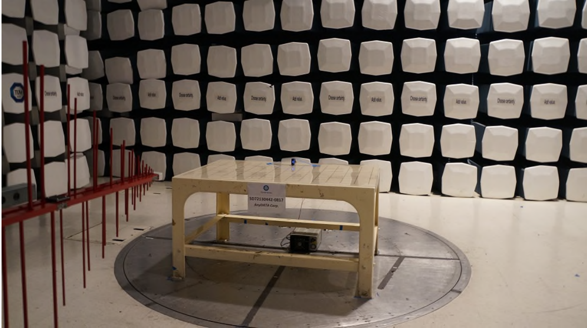
Radiated Emissions Below 1GHz Front
