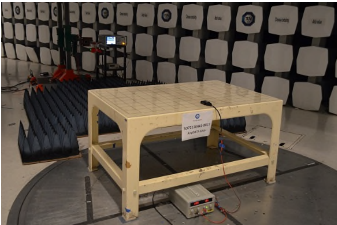
Radiated Emissionsv Above 1GHz Rear
