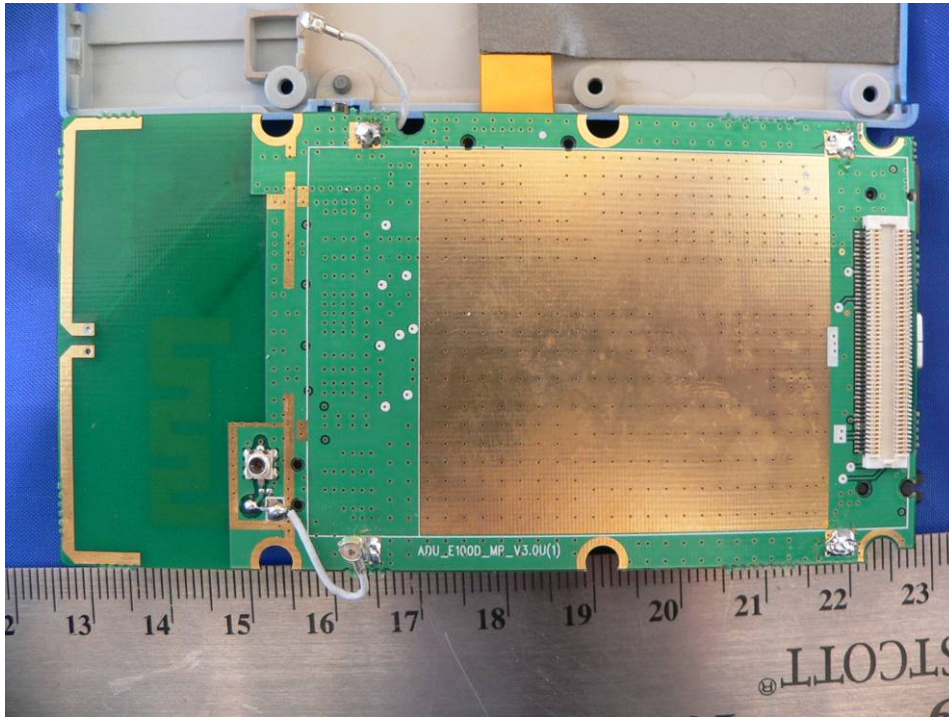
EUT – Components view 3
