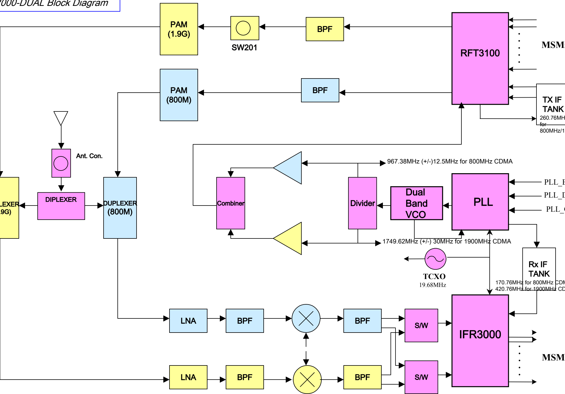
000-DUAL Block Diagram
