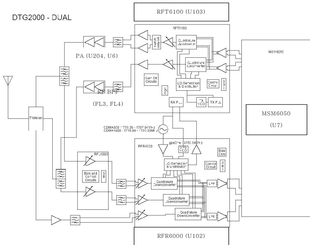
Figure 1. DTG2000-DUAL Block Diagram
