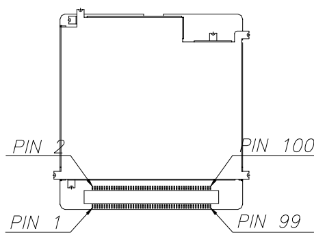
100 PIN ASSIGNMENT
