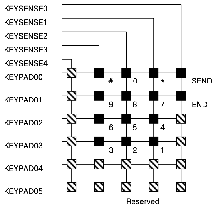
Figure 4-1 Keypad Matrix
