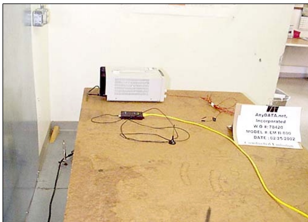
AC Conducted Emissions Test Setup - Back View
