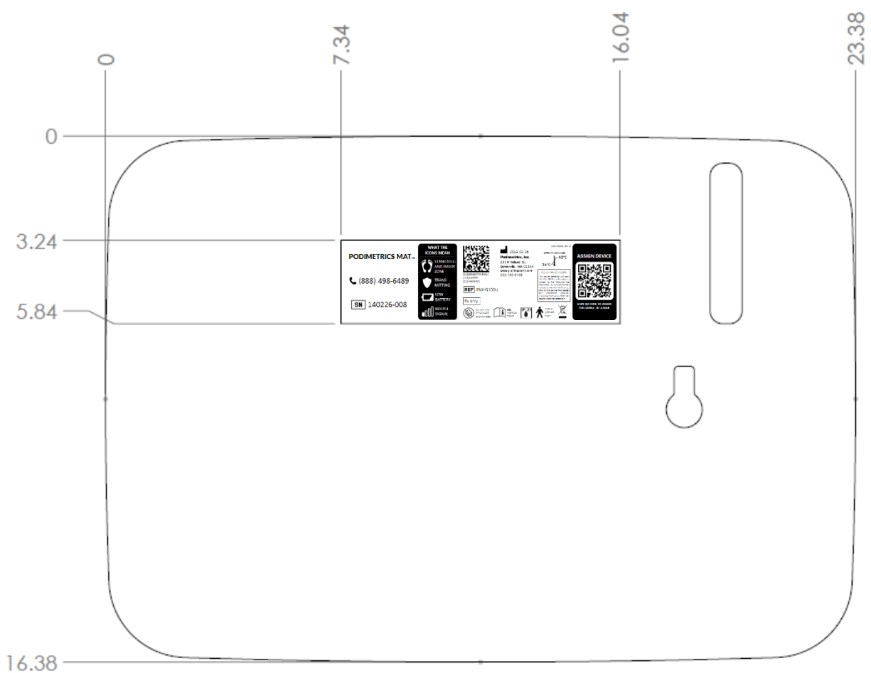
Label on bottom of device (all dimensions are in inches)
